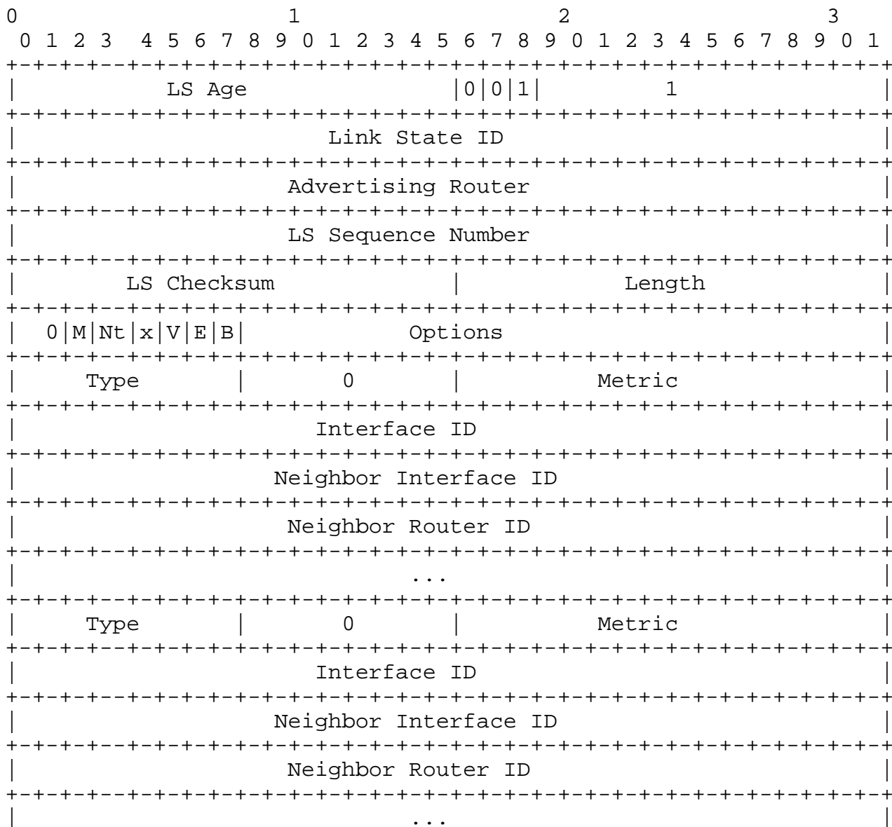
M-bit in OSPFv3 Router LSA
