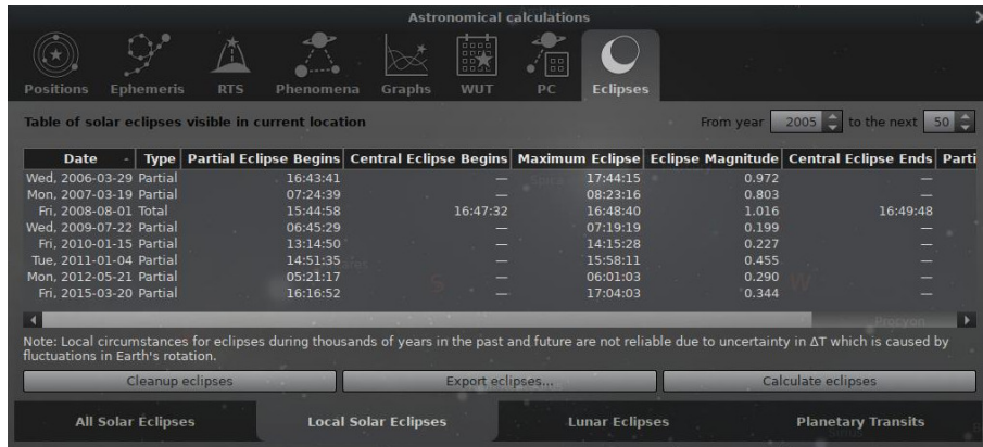
Figure 4.43: Astronomical Calculations (AstroCalc): Eclipses / Local Solar Eclipses
